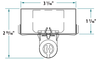
Fixture Housing Dimensions
