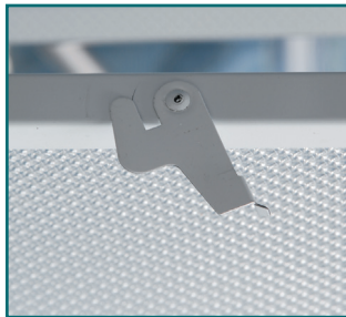
Cam Latch (Secured to Frame Door) (Provides Quick Access to Lamps/Ballasts)
